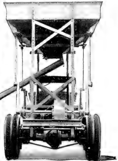
Above: Four jointed steel arms raise this steel coal body ten feet in thirty seconds
